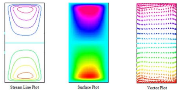
Figure 19. Streamline plot, surface plot, and vector plot of the secondary flow for rotating straight duct of rectangular cross-section at R=75 and aspect ratio \sigma = 2 with pressure driven parameter P_n = 100 .
