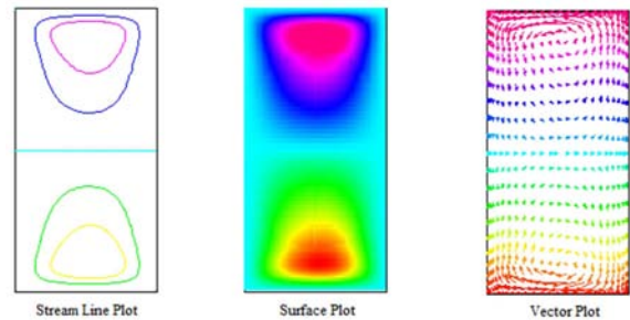
Figure 11. Streamline plot, surface plot, and vector plot of the secondary flow for rotating straight duct of rectangular cross-section at R=40 and aspect ratio \sigma =2 with pressure driven parameter P_n =100 .
