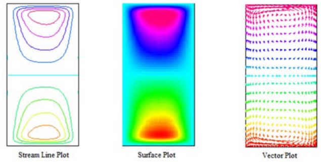
Figure 17. Streamline plot, surface plot, and vector plot of the secondary flow for rotating straight duct of rectangular cross-section at R=70 and aspect ratio \sigma = 2 with pressure driven parameter P_n = 100 .
