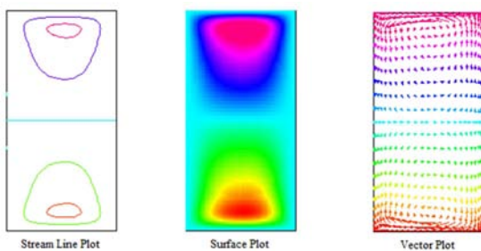
Figure 15. Streamline plot, surface plot, and vector plot of the secondary flow for rotating straight duct of rectangular cross-section at R=60 and aspect ratio \sigma = 2 with pressure driven parameter P_n = 100 .
