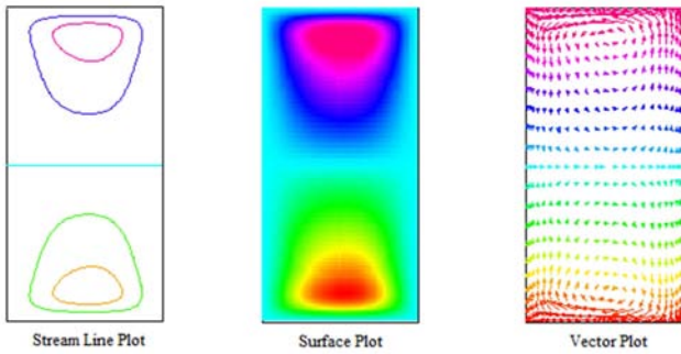
Figure 13. Streamline plot, surface plot, and vector plot of the secondary flow for rotating straight duct of rectangular cross-section at R=50 and aspect ratio \sigma = 2 with pressure driven parameter P_n = 100 .
